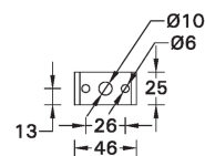
MOUNTING DETAIL
