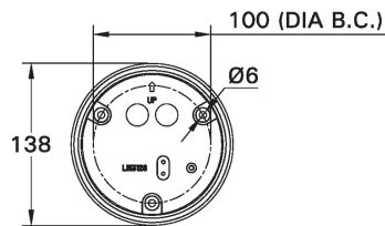
MOUNTING DETAIL
