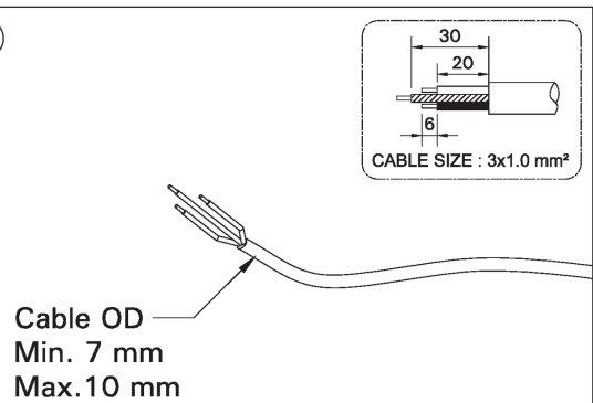
MOUNTING DETAIL
