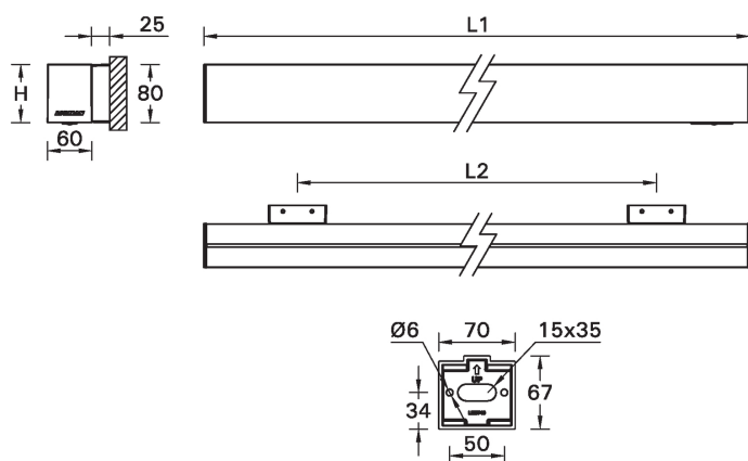
MOUNTING DETAIL
