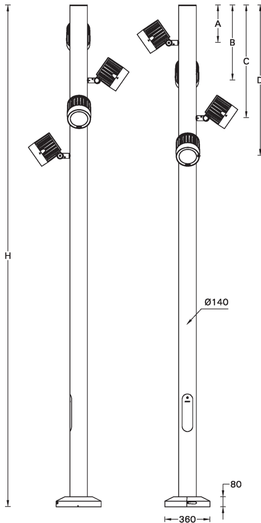
Mounting detail
