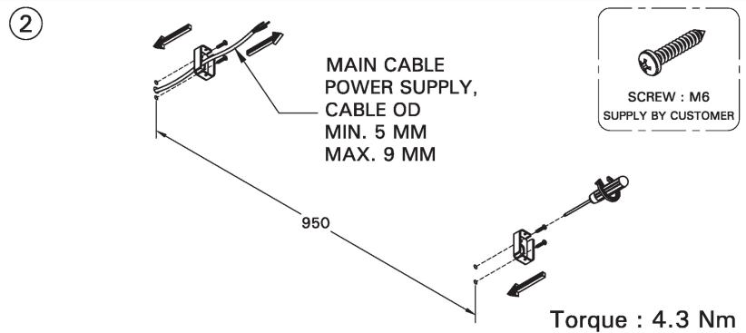
MOUNTING DETAIL
