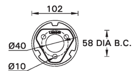
MOUNTING DETAIL
