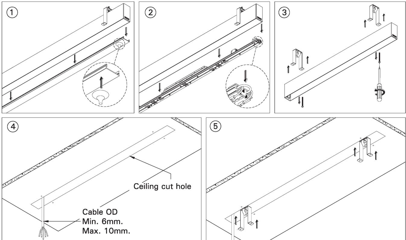
MOUNTING DETAIL
