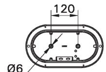
MOUNTING DETAIL
