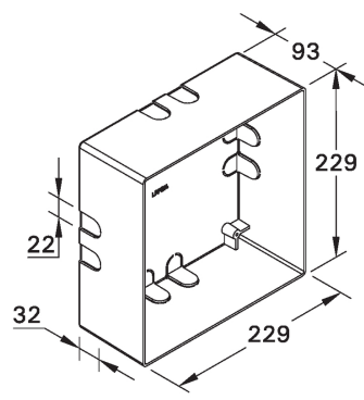
RECESSING BOX
