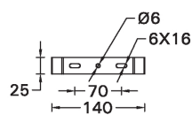
MOUNTING DETAIL
