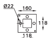
MOUNTING DETAIL
