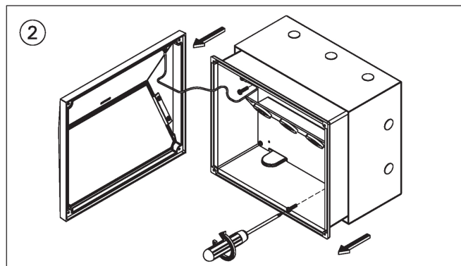
RECESSING BOX
