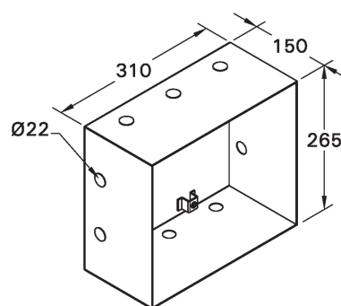
RECESSING BOX
