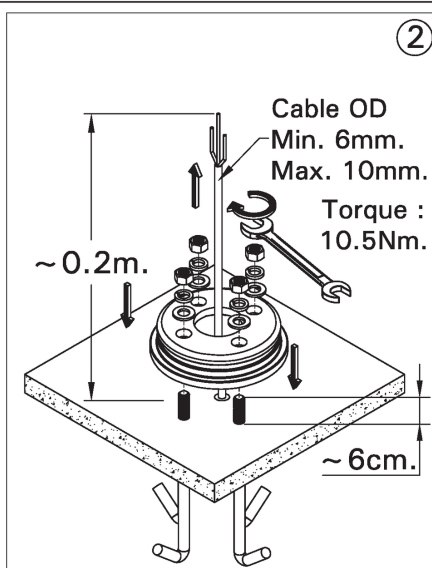
MOUNTING DETAIL
