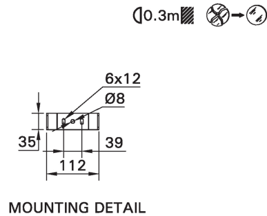
MOUNTING DETAIL
