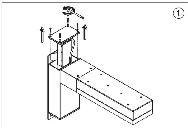
MOUNTING DETAIL
