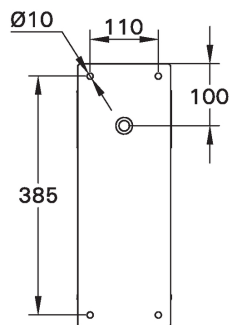
MOUNTING DETAIL
