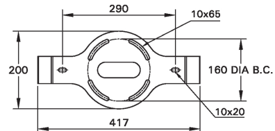
MOUNTING DETAIL QA-50021
