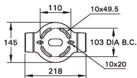
MOUNTING DETAIL QA-50001,QA-50003
