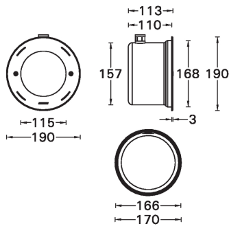
MOUNTING DETAIL BOH-60022
