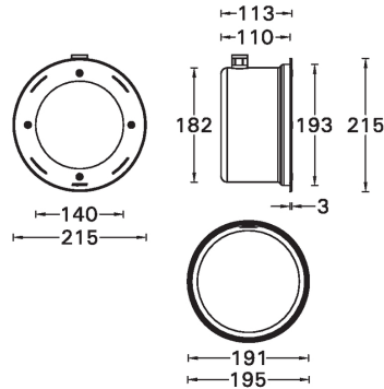
MOUNTING DETAIL BOH-60032
