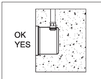
MOUNTING DETAIL BOH-60022
