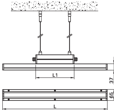
Mounting detail
