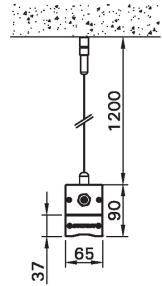
Mounting detail
