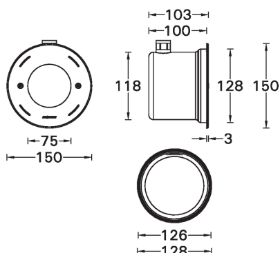
MOUNTING DETAIL BOH-60013
