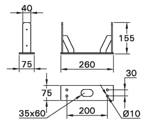
MOUNTING DETAIL
