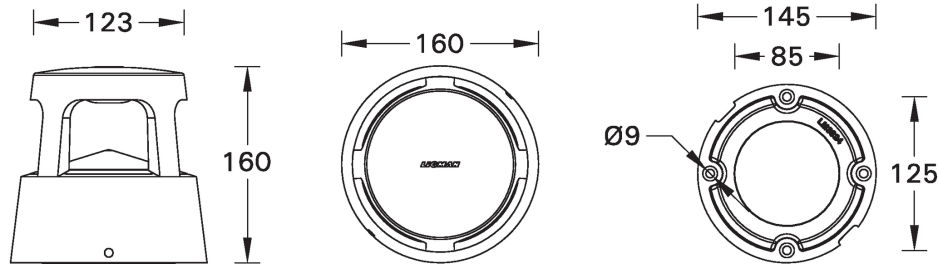
MOUNTING DETAIL
