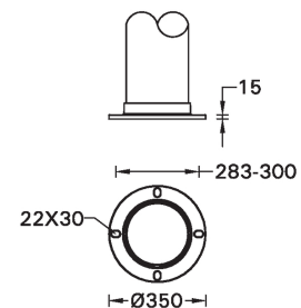
MOUNTING DETAIL
