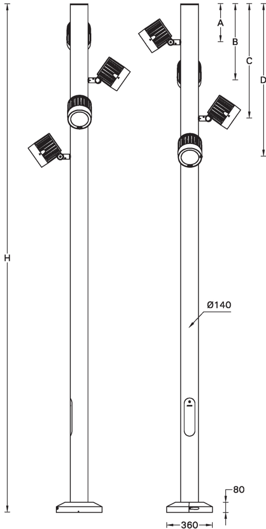
Mounting detail
