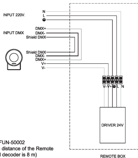
REMOTE BOX
