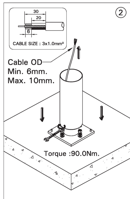
MOUNTING DETAIL
