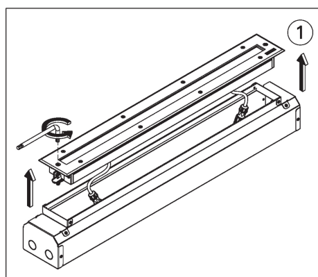
MOUNTING DETAIL
