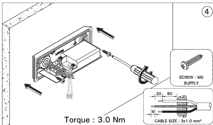
MOUNTING DETAIL
