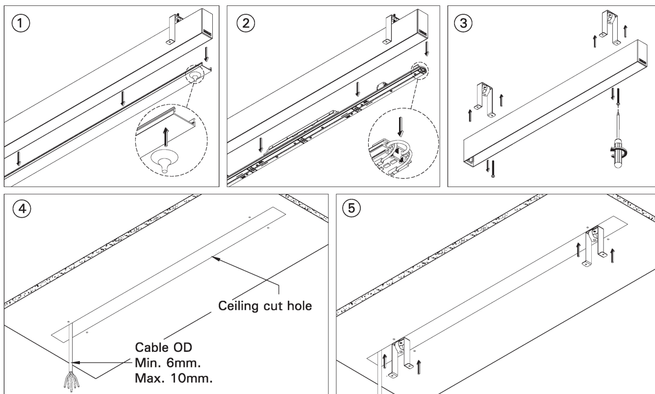
MOUNTING DETAIL
