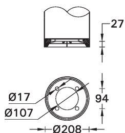
MOUNTING DETAIL
