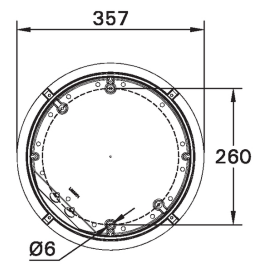
MOUNTING DETAIL
