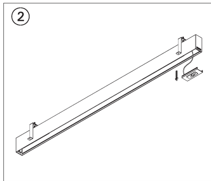
MOUNTING DETAIL
