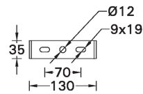
MOUNTING DETAIL NOD-50032
