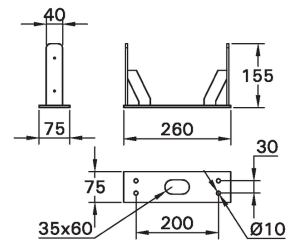
MOUNTING DETAIL
