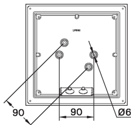
MOUNTING DETAIL
