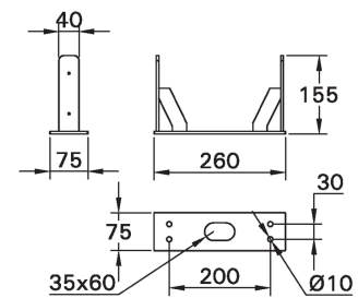
MOUNTING DETAIL
