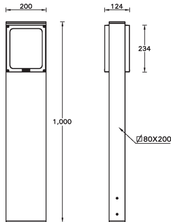
VT-10011, VT-10012
