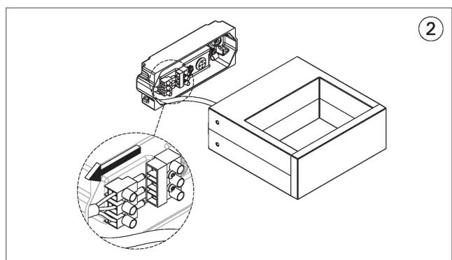
MOUNTING DETAIL AUG-30021
