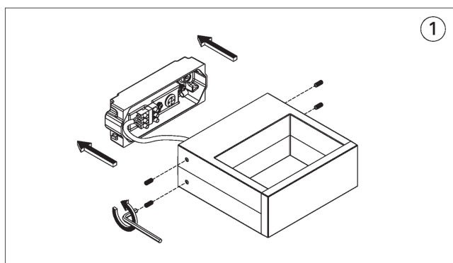
MOUNTING DETAIL AUG-30011
