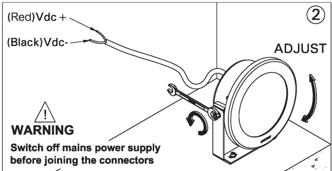
MOUNTING DETAIL
