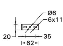
MOUNTING DETAIL
