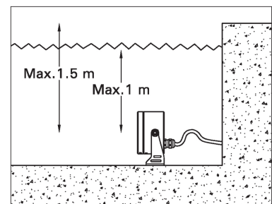
MOUNTING DETAIL
