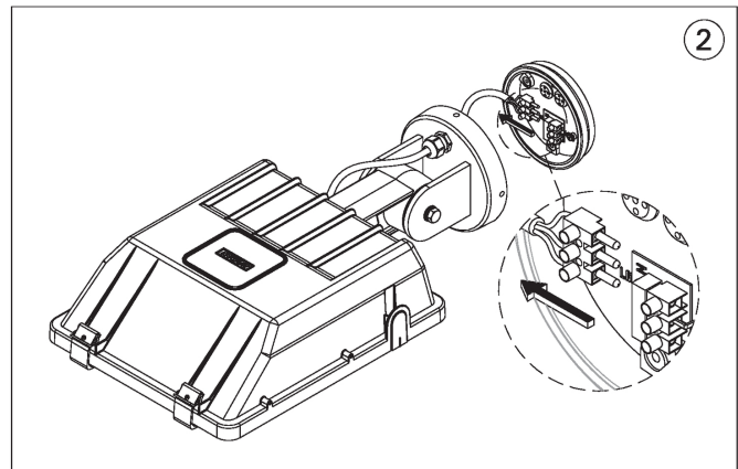
MOUNTING DETAIL
