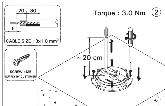
MOUNTING DETAIL
