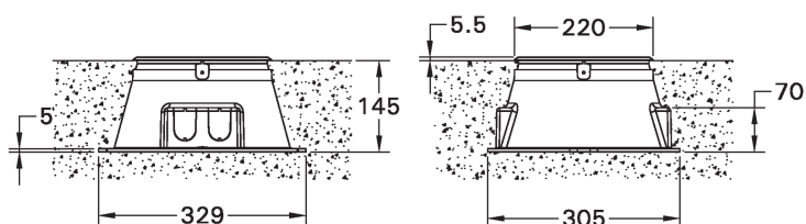
FRONT SURFACE RING KI-60445
