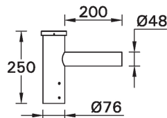
A90560 FOR SC60 Single arm mounting
