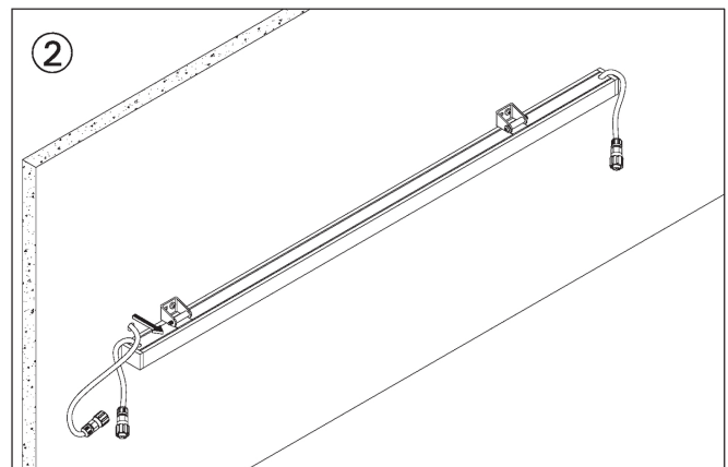
MOUNTING DETAIL
