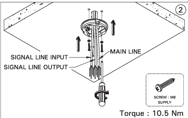
MOUNTING DETAIL
