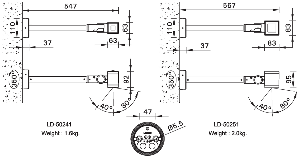
Mounting detail
