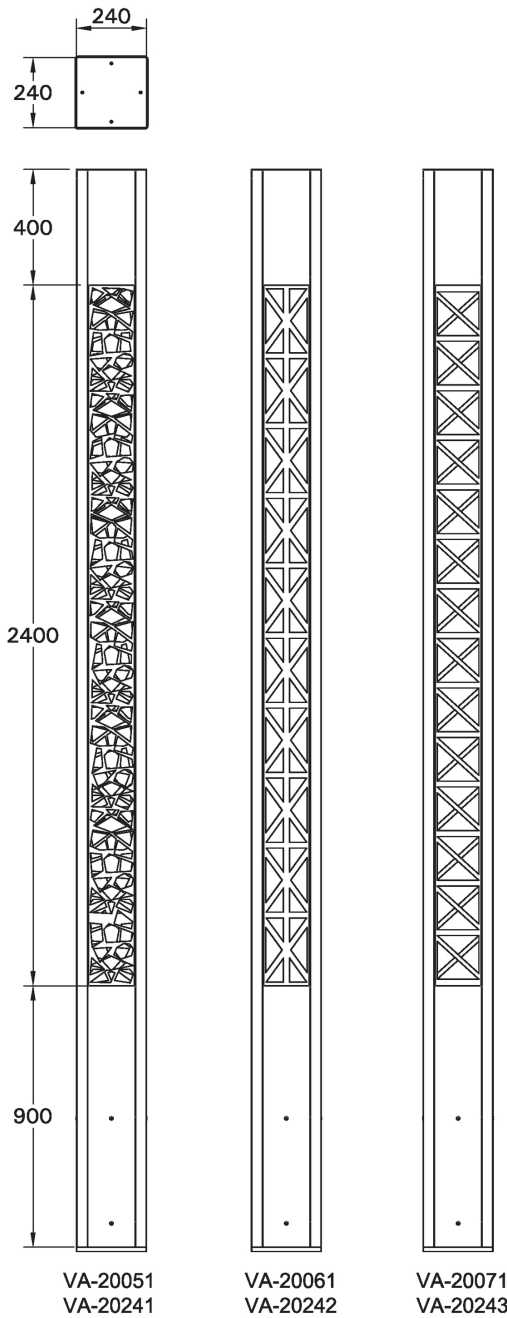
MOUNTING DETAIL
