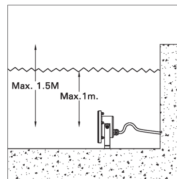
MOUNTING DETAIL
