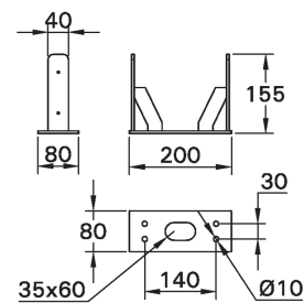
MOUNTING DETAIL
